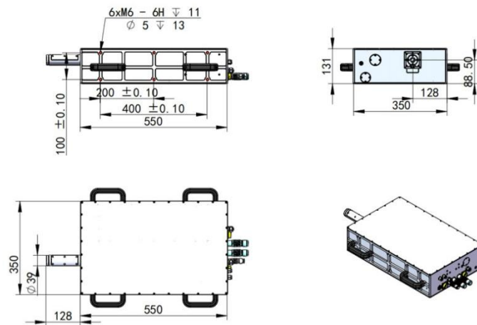
laser Head
