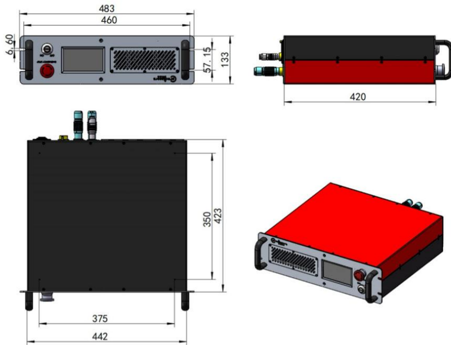
Laser Controller
